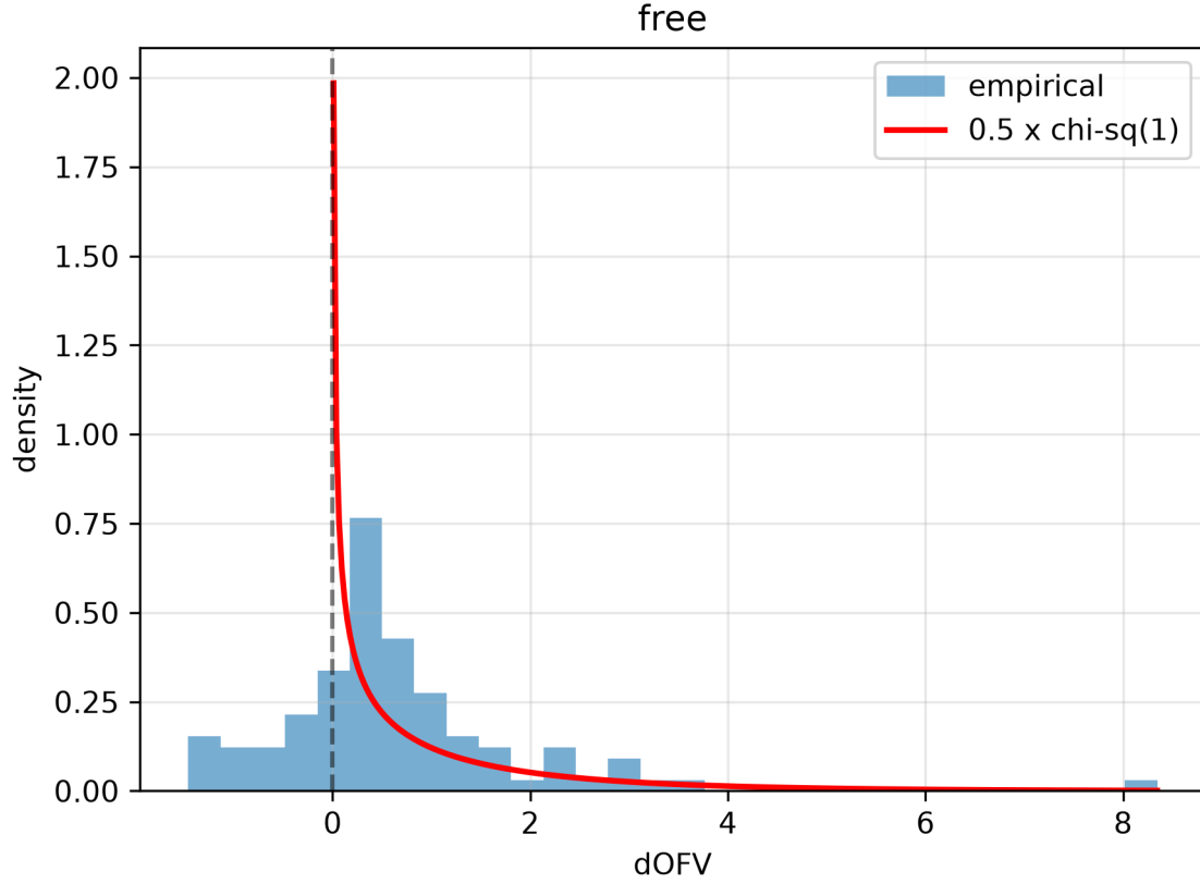
Empirical \Delta\text{OFV} distribution under the null hypothesis, free versus amortized posterior, against the theoretical Self-Liang mixture reference density.
