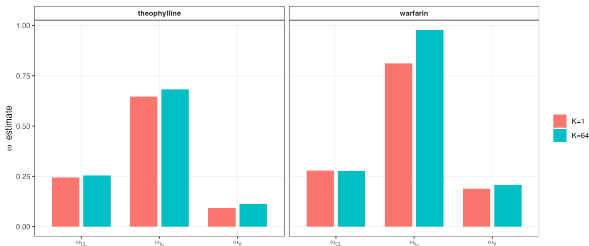
Figure 4: between-subject variability estimates at K = 1 versus K = 64 for each dataset, by parameter.
