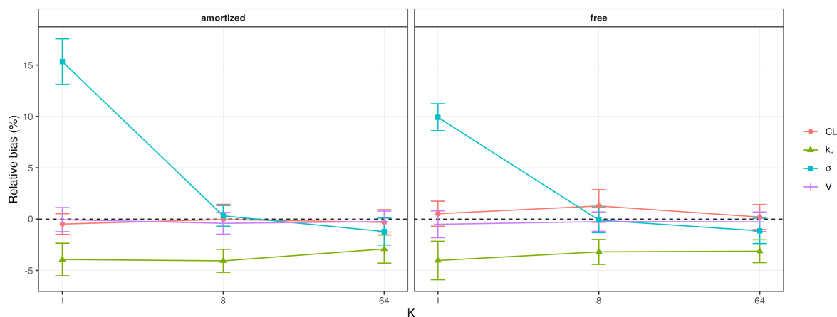
Figure S1: Structural fixed-effect and residual-error bias by K , shown separately for free and amortized posteriors in the Phase 0 Gaussian analysis. The dashed line marks zero bias; error bars show the standard error across replicates.
