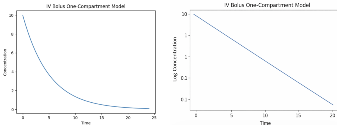
Figure 6: 1cpt bolus lin log
