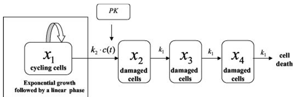
Figure 11: simeoni tgi
