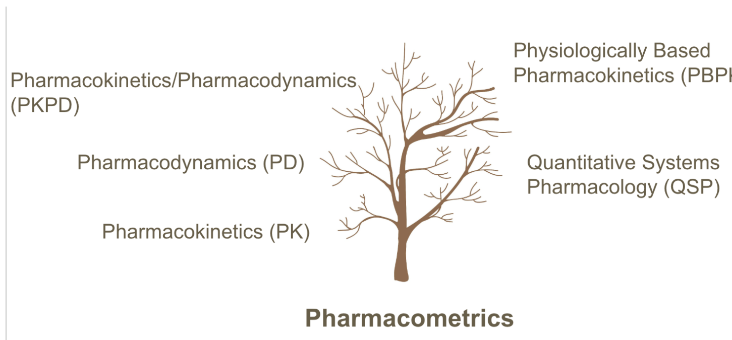
Figure 1: pmx tree
