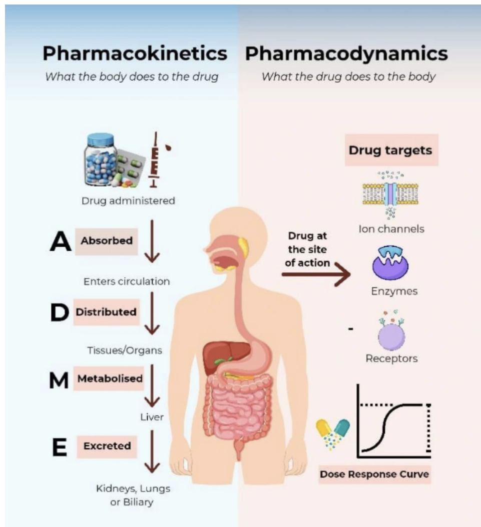
Figure 2: pkpd diagram
