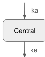
Figure 7: 1cpt oral
