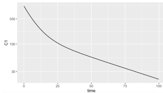
Figure 9: 2cpt bolus
