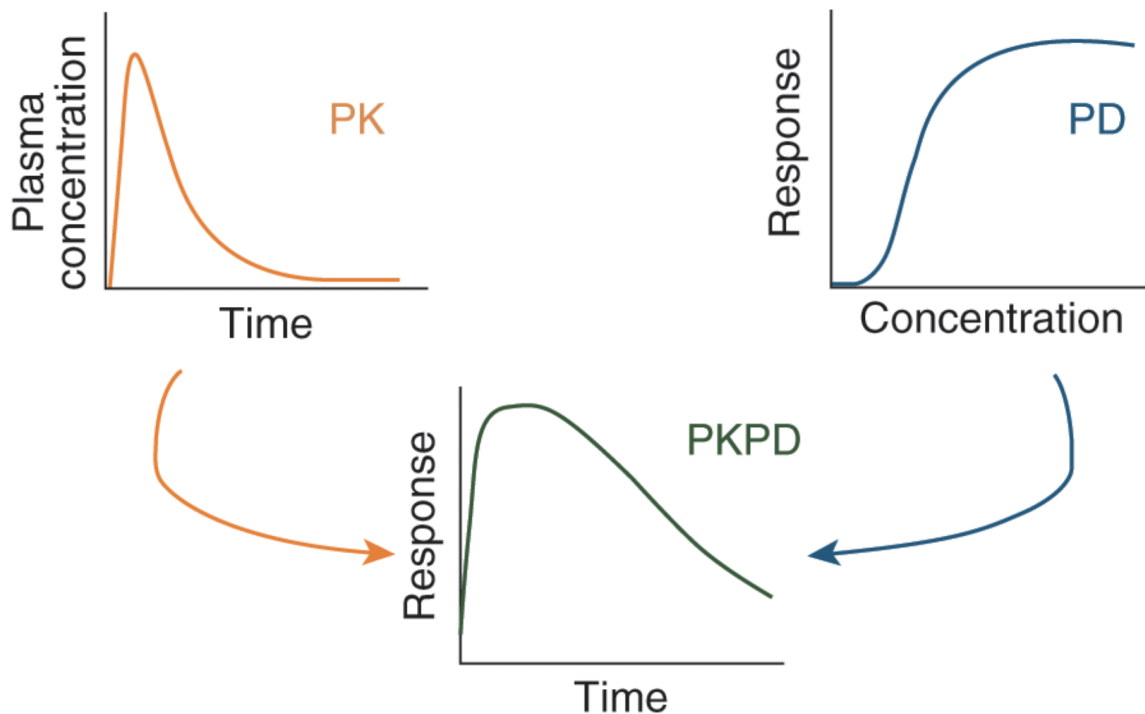
Figure 3: pkpd plots concept
