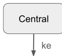
Figure 5: 1cpt iv
