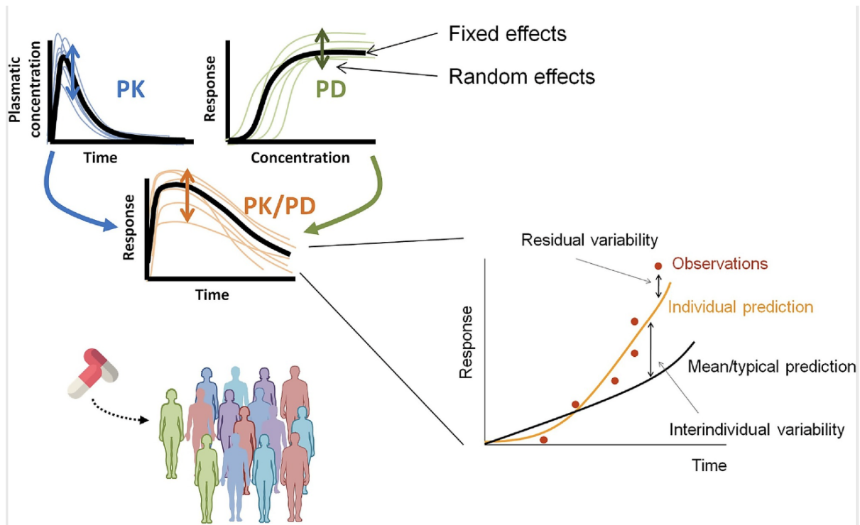
Figure 10: nlme
