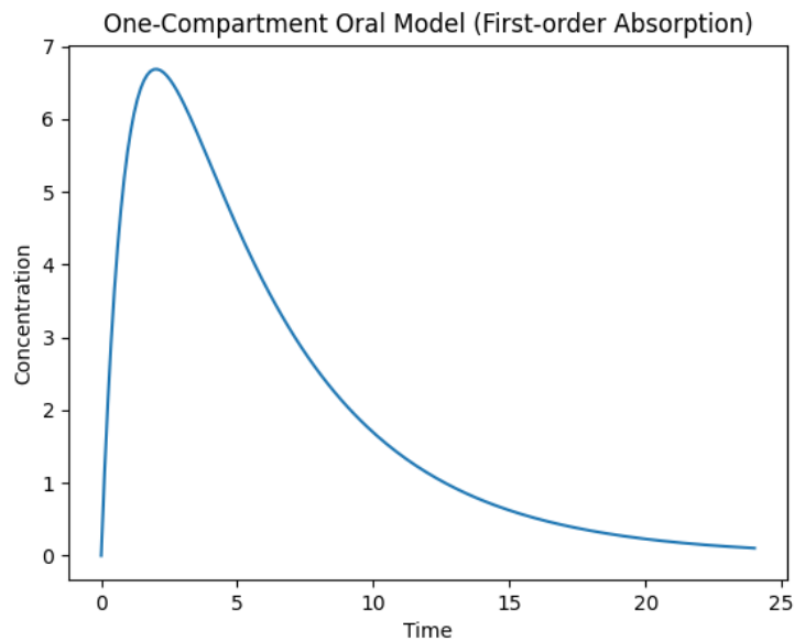
Figure 8: oral model
