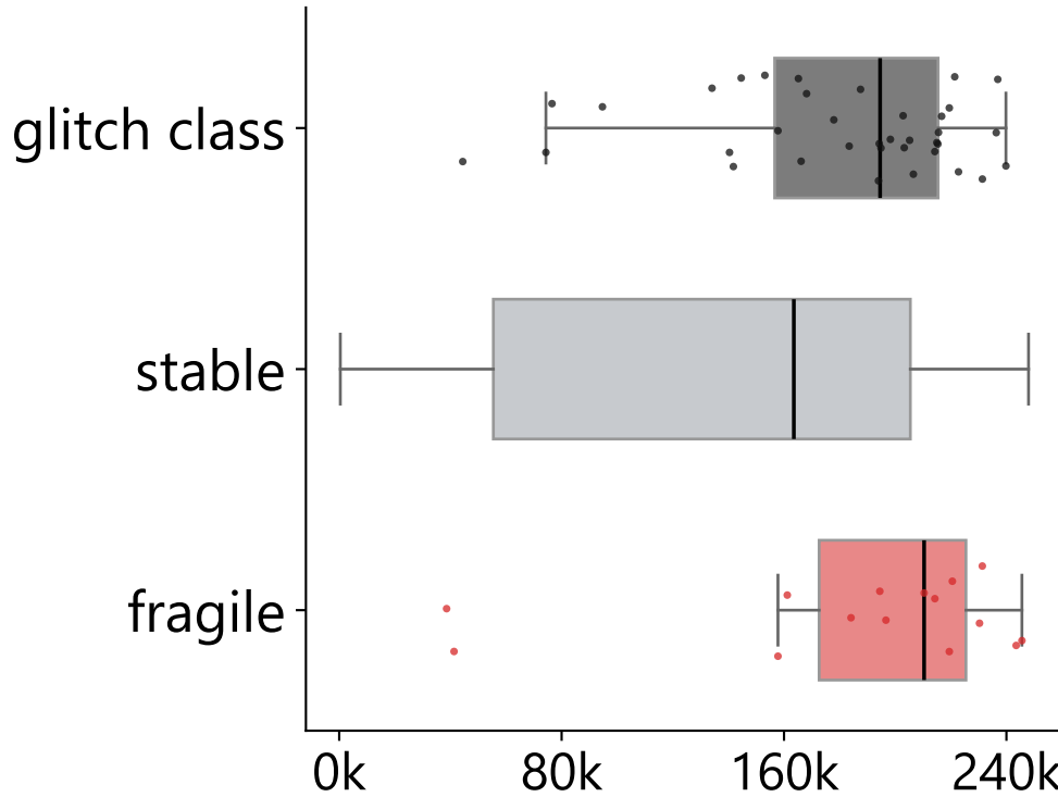
Qwen3.8-Flash-Next
