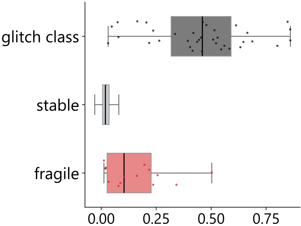
Qwen3.8-Flash-Next
