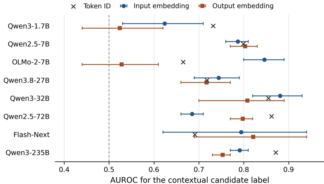
Figure 1. Geometric association with the contextual candidate label. Points and horizontal bars show the reported proximity AUROC and 95% bootstrap interval in each embedding space. Crosses show the token-ID score. The line at 0.5 marks chance ranking. The model-wise choice of the stronger space is descriptive. Sample counts and the remaining geometric scores appear in Table B1.
