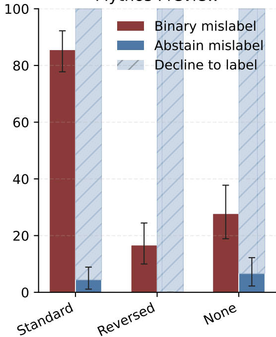
Mythos Preview
