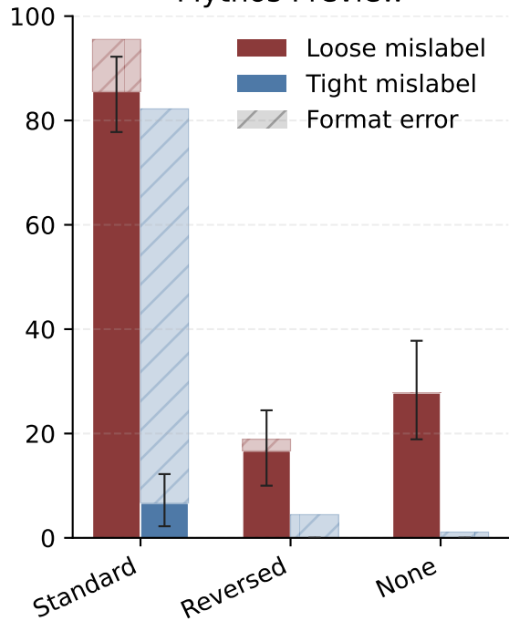
Mythos Preview
