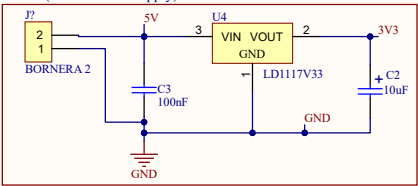
Power (5V 2A Power Supply)
