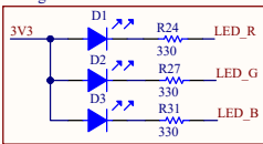
Debug LEDs
