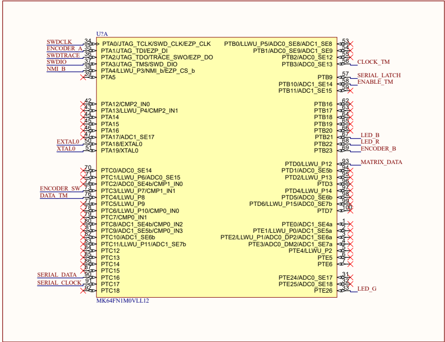
K64F Microcontroller
