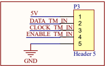
Card Reader
