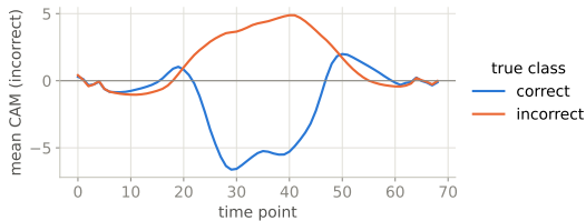
Mean CAM for incorrect , grouped by true class.
