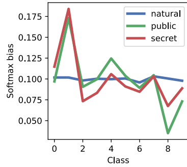
(a) Softmax biases for each class
