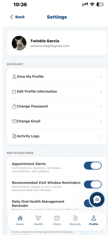
Figure 183. Settings (Mobile)
