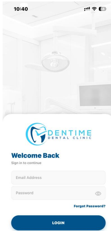
Figure 136. Login (Mobile)
