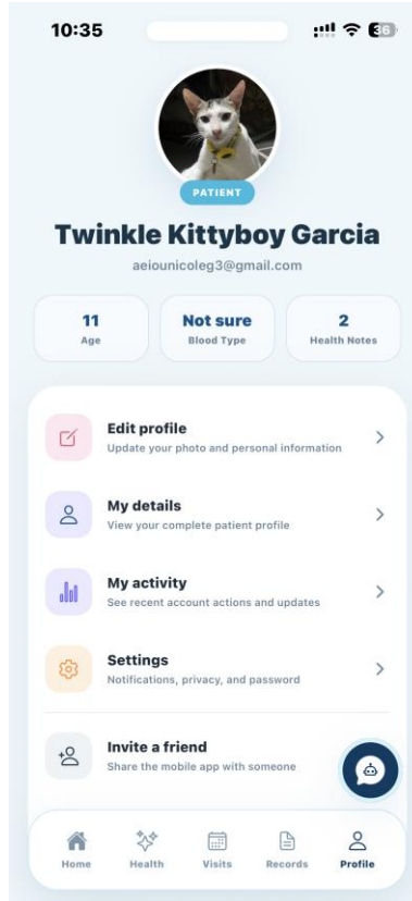
Figure 179. Profile (Mobile)
