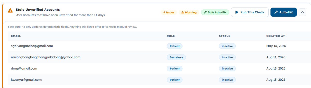
Figure 115. Integrity Tools - Stale Unverified Accounts (Web)
