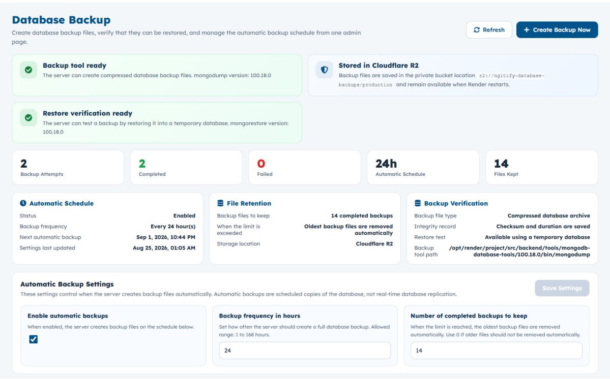
Figure 110. Database Backup (Web)
