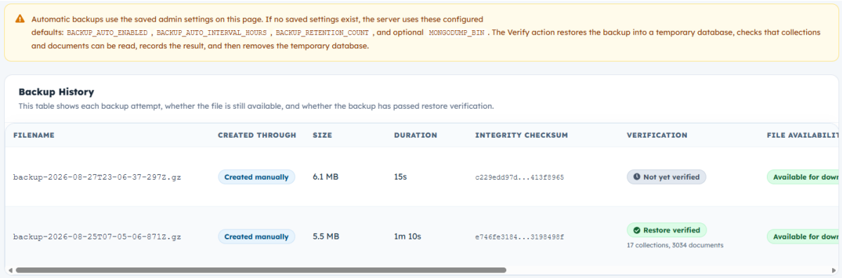
Figure 111. Database Backup History (Web)
