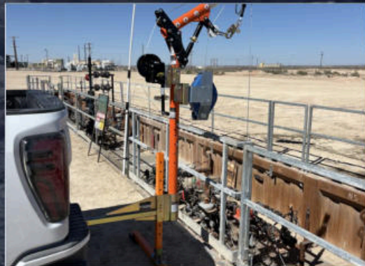
DAVIT RESCUE SYSTEMS — TRUCK-MOUNTED, READY TO RIG
