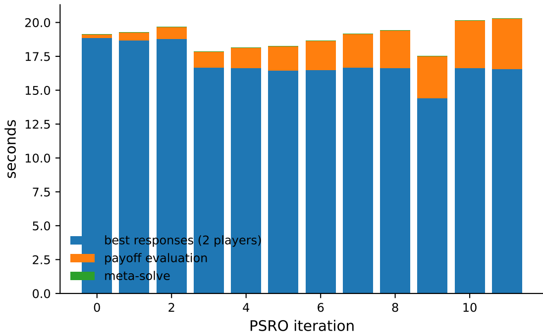
Where each iteration's time goes
