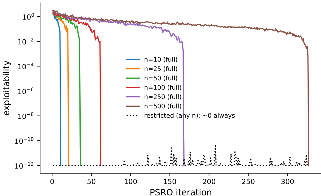
Full-game exploitability falls; restricted says 'done' immediately
