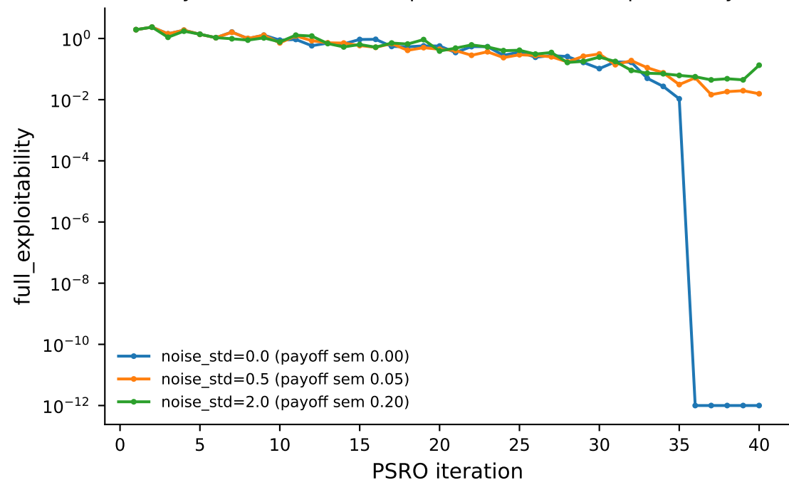
Payoff-estimation noise puts a floor under exploitability
