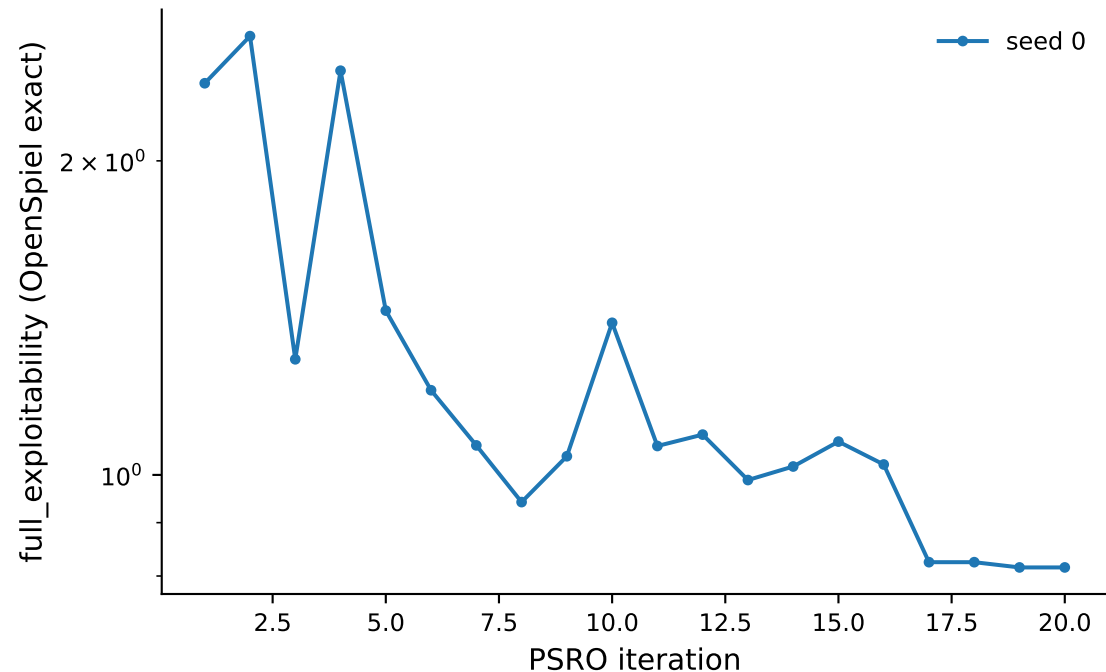
Leduc poker: PSRO with Nash meta-solver + PPO oracle
