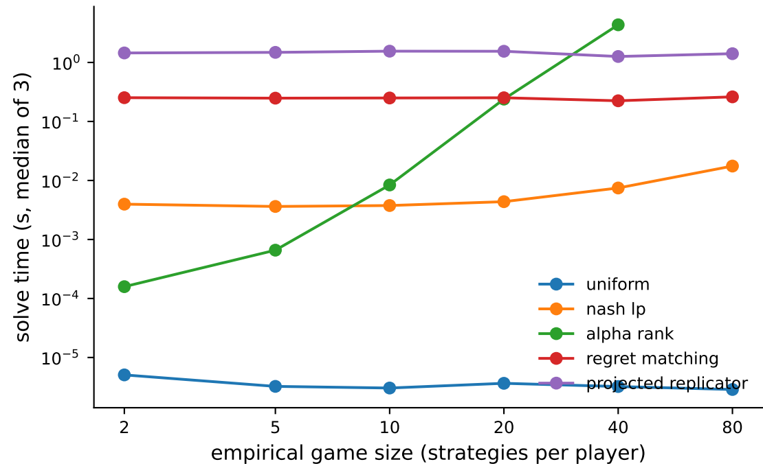
Meta-solver cost as the population grows
