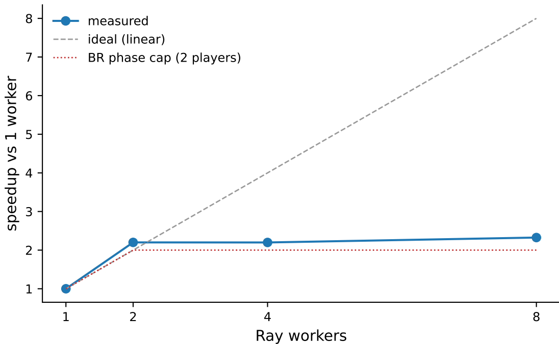
Parallel PSRO on Leduc: Amdahl bites at 2 workers
