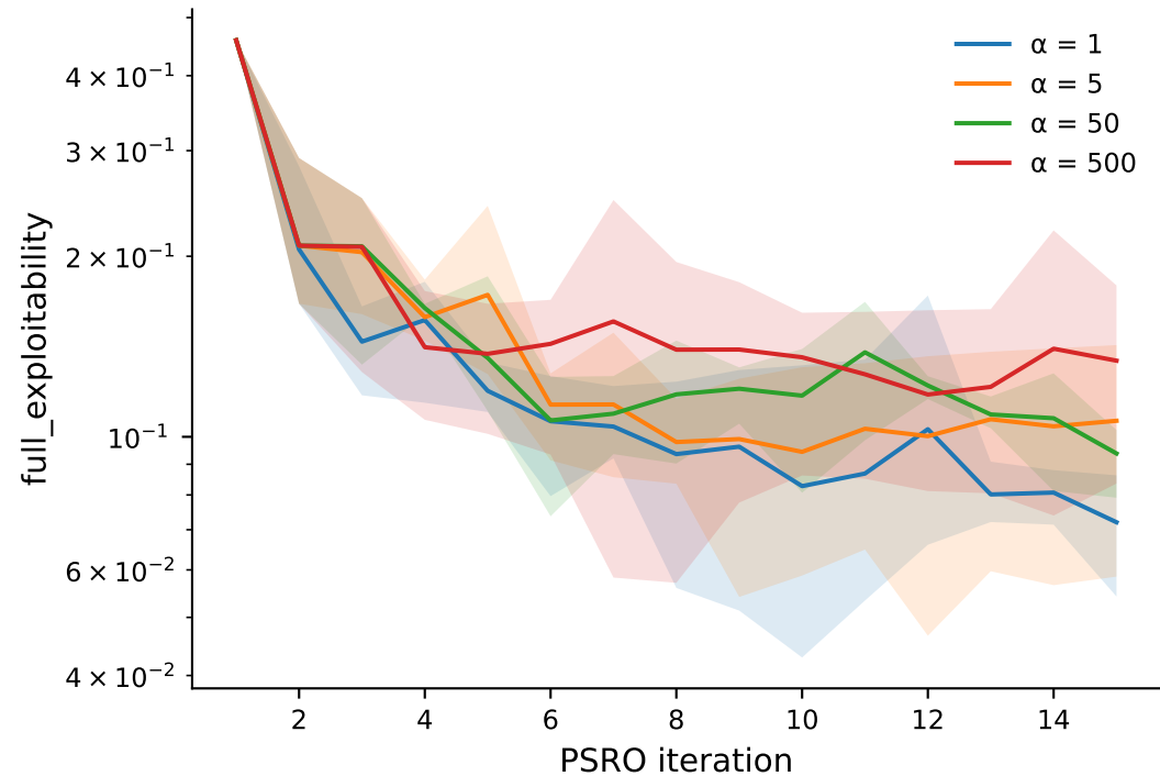
\alpha -sweep: exploitability
