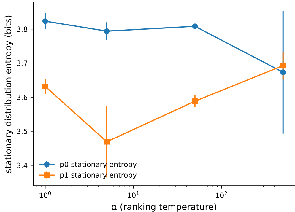
\alpha \downarrow \rightarrow uniform; \alpha \uparrow \rightarrow sink concentration
