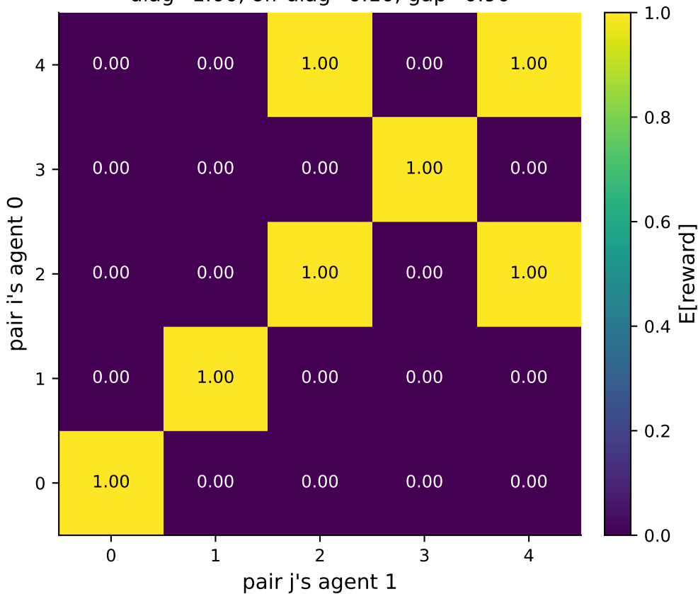
Joint-policy correlation on a 5-colour matching game diag=1.00, off-diag=0.10, gap=0.90
