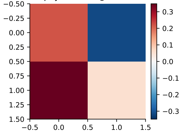
payoff table @ iter 1
