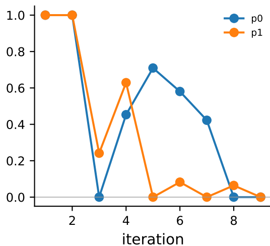
newest member mass
