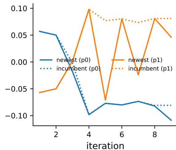
BR value vs incumbent
