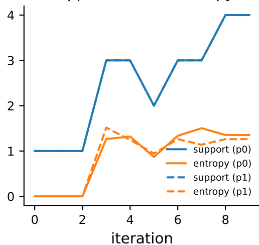
support size and entropy
