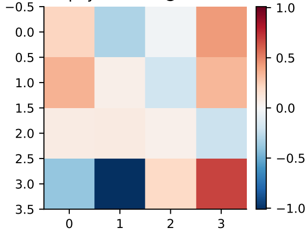
payoff table @ iter 3
