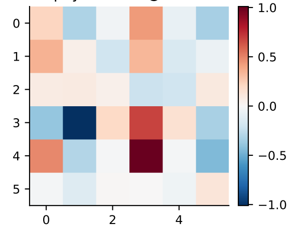
payoff table @ iter 5
