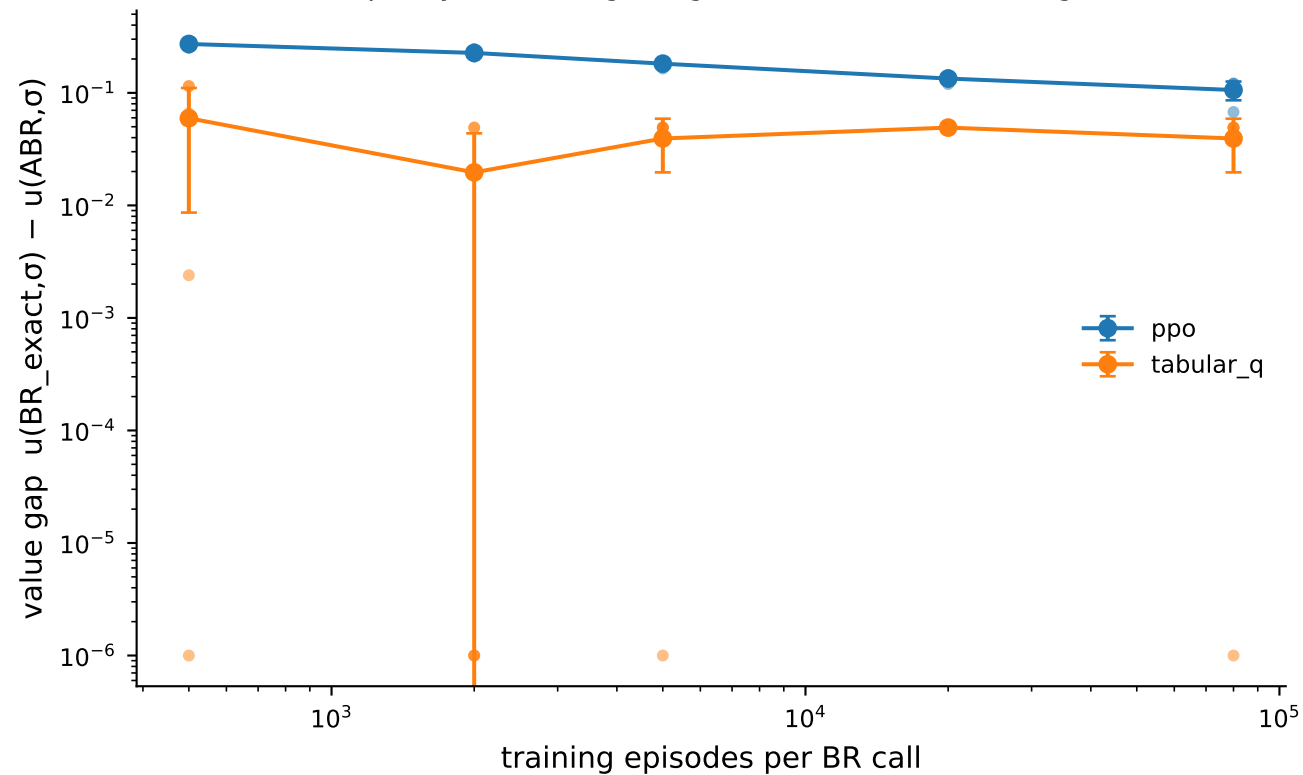
BR quality vs training budget (shared reference target)
