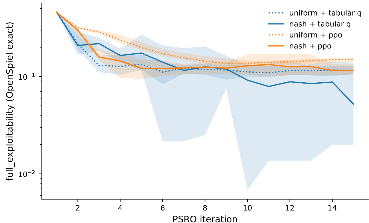
Kuhn poker: Nash meta-solver ahead for both oracles; exact-ish tabular BRs beat PPO's approximate ones
