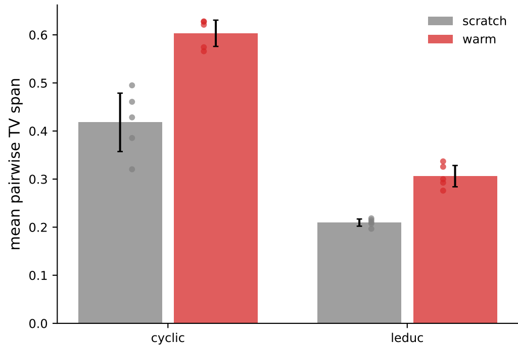
Warm-started PPO best responses vs from-scratch (Ch. 12 §12.4)
