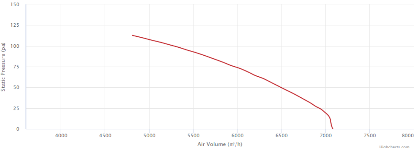
50GSC_230V 60Hz
