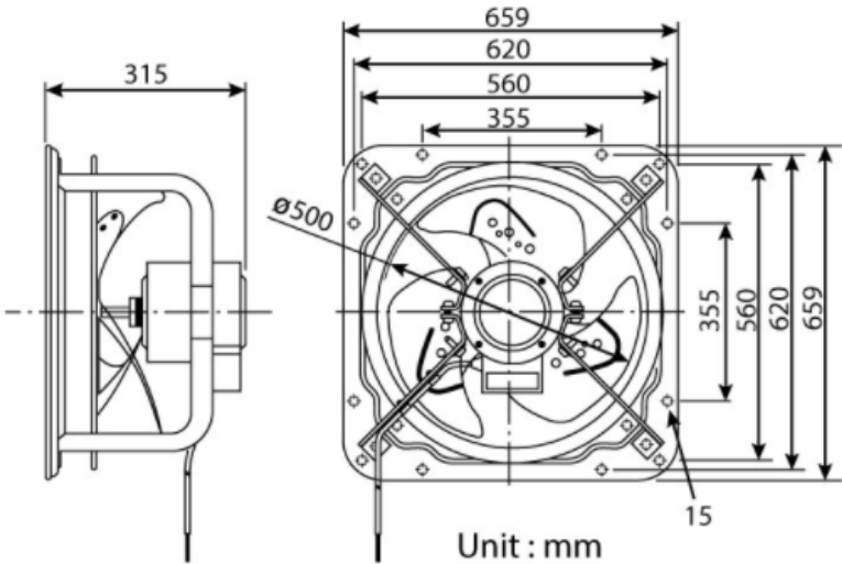
50GSC Dimension
