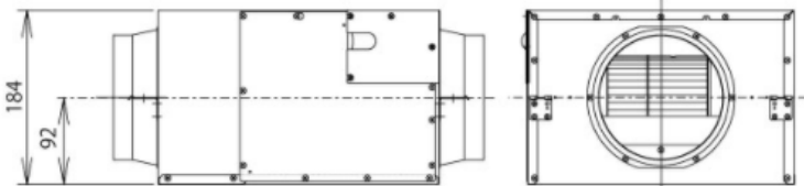
12NSB Dimension
