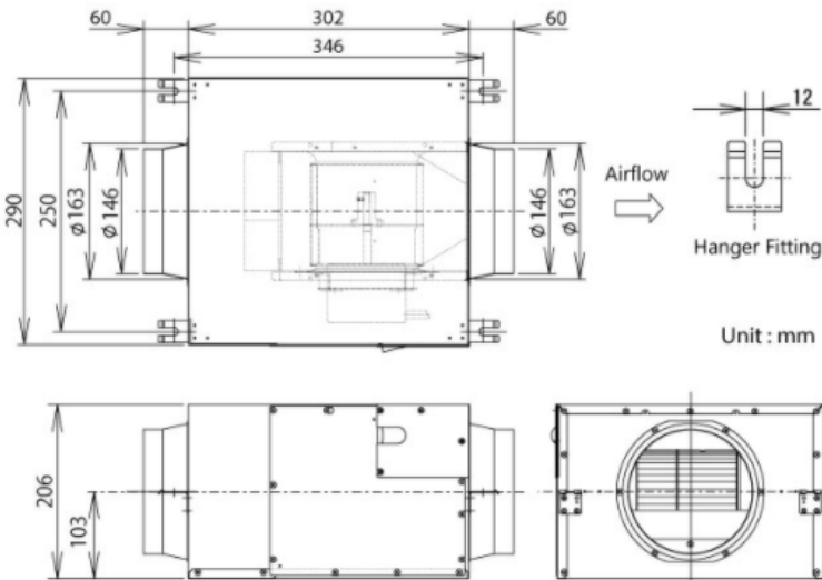
15NSB Dimension
