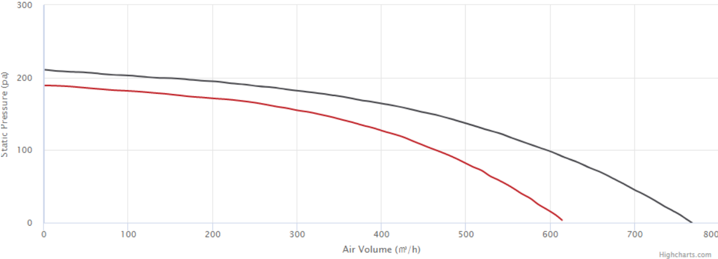
18NFB_230V 50Hz
