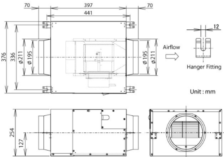
18NFB_230V 50Hz
