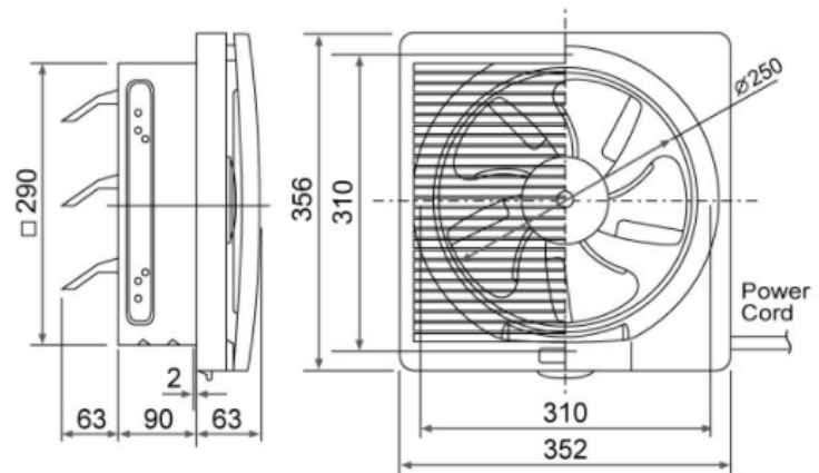
25RLF Dimension
