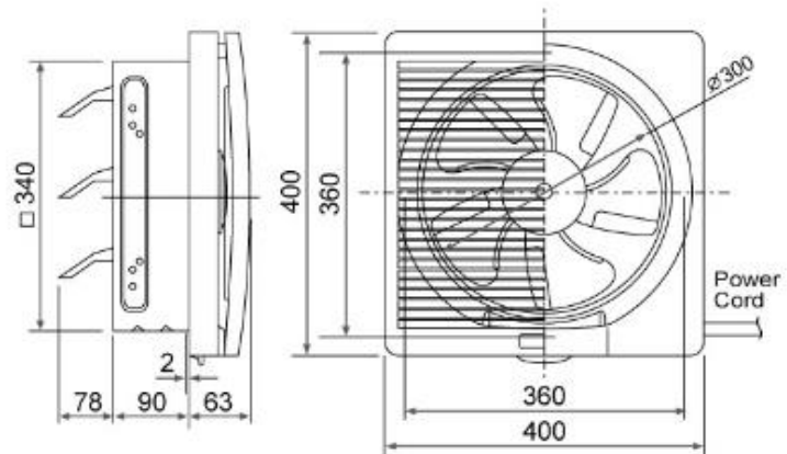
30RLE Dimension
