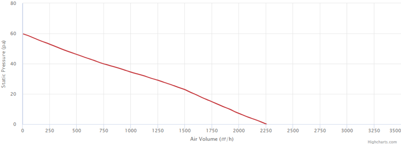
40KQT_230V 60Hz
