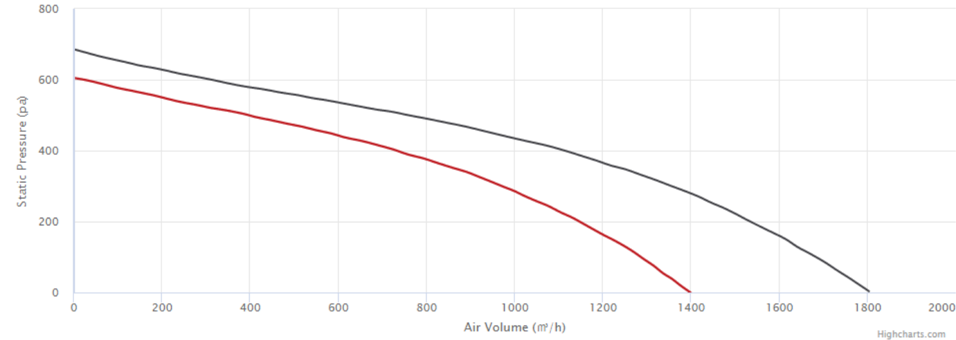
25NFB_220V 60Hz
