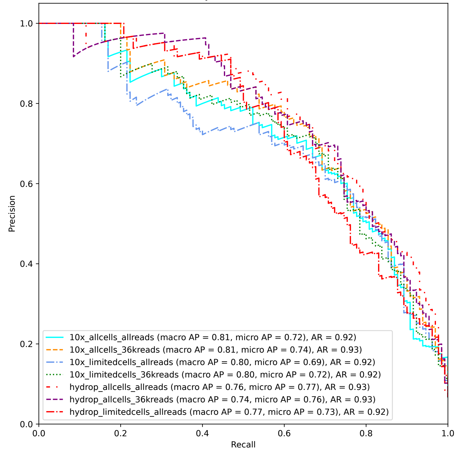
Summary Precision-Recall Curve
