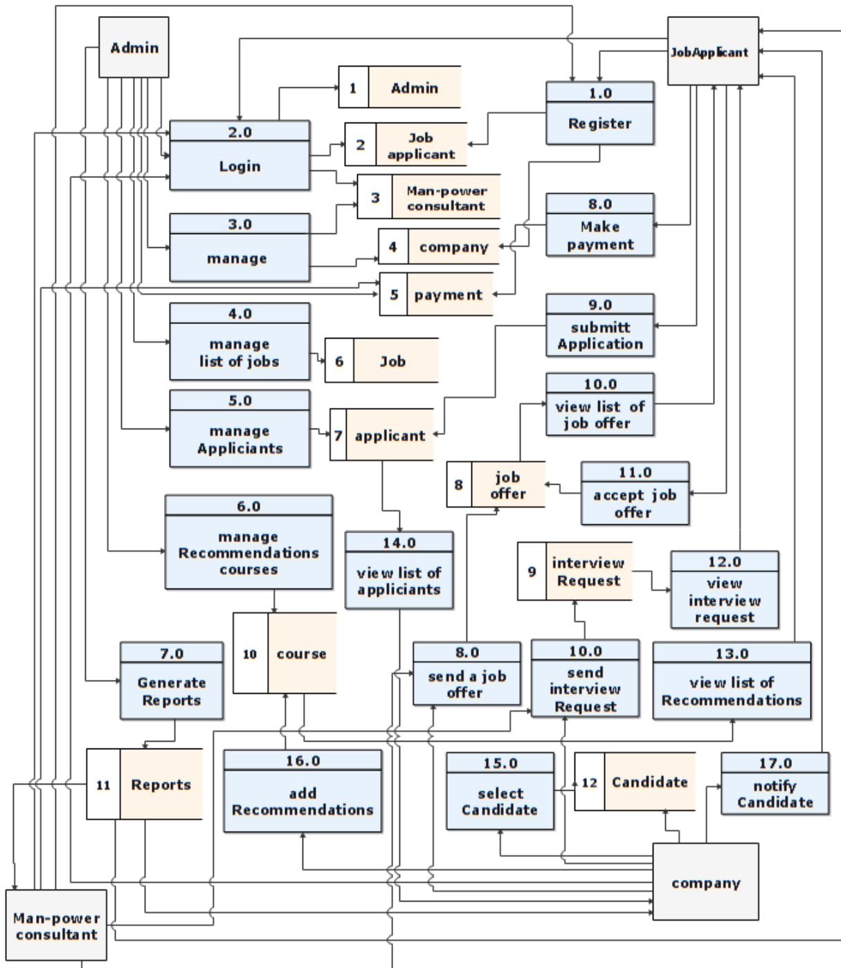
Figure 3.29. DFD diagram
