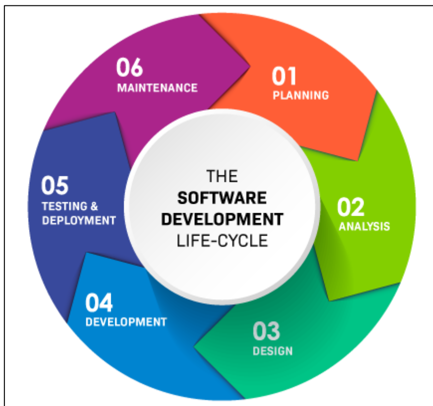
Figure 3.1. SDLC
