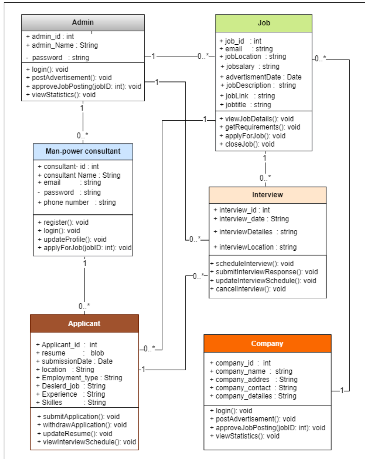
Figure 3.31. Class Diagram
