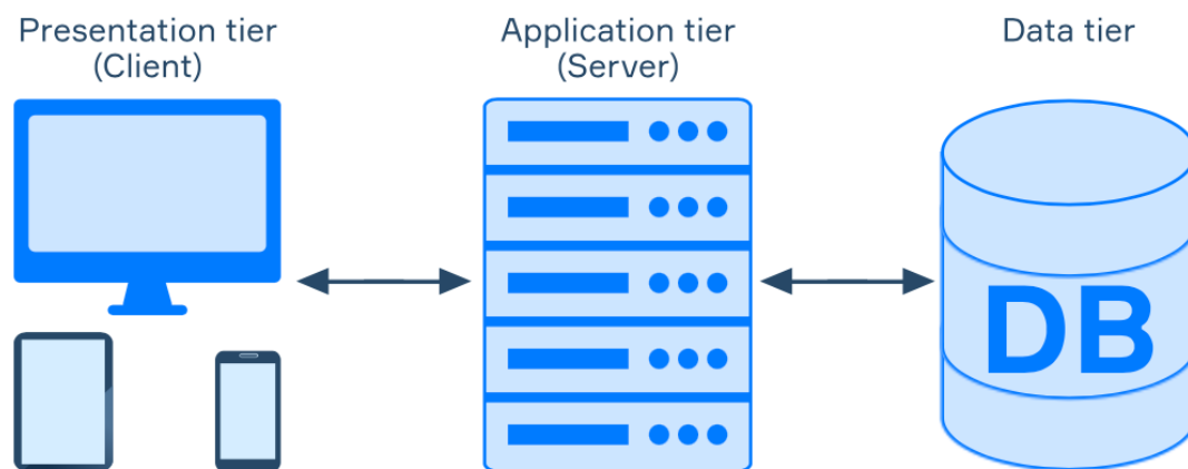
Figure 1.1. System Architecture
