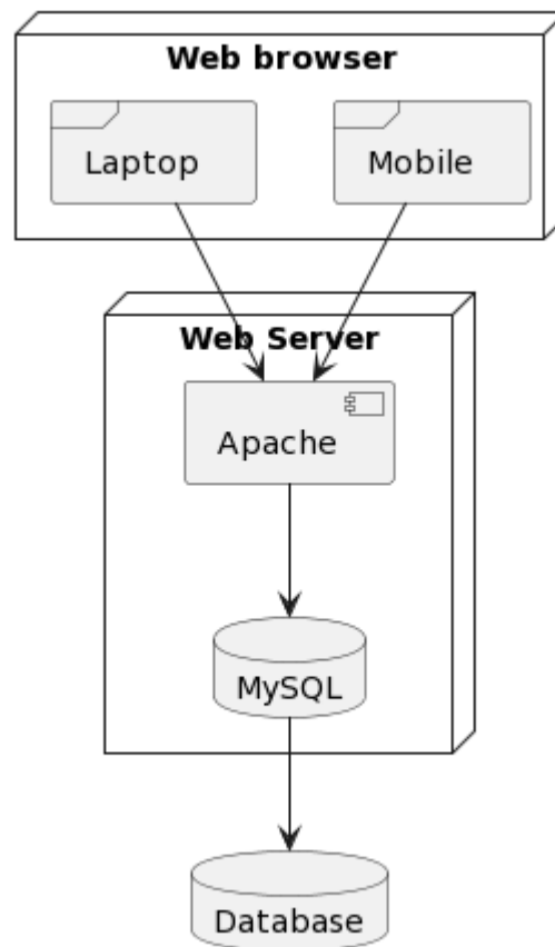
Figure 3.32. Deployment Diagram
