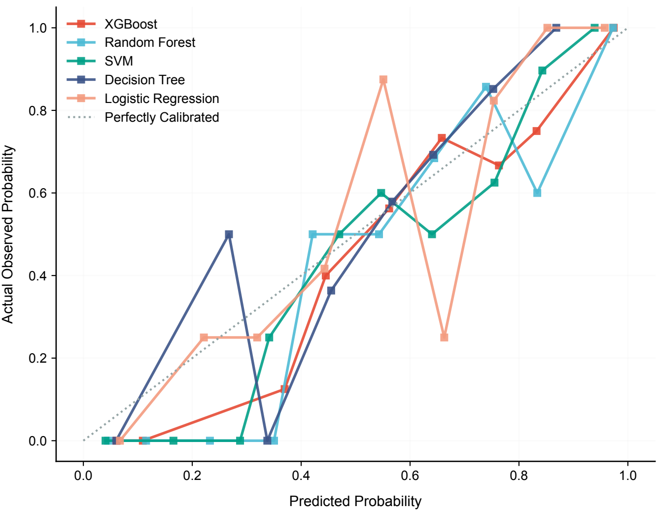
Calibration: COMPOSITE (Subgroup No Renal = 0)
