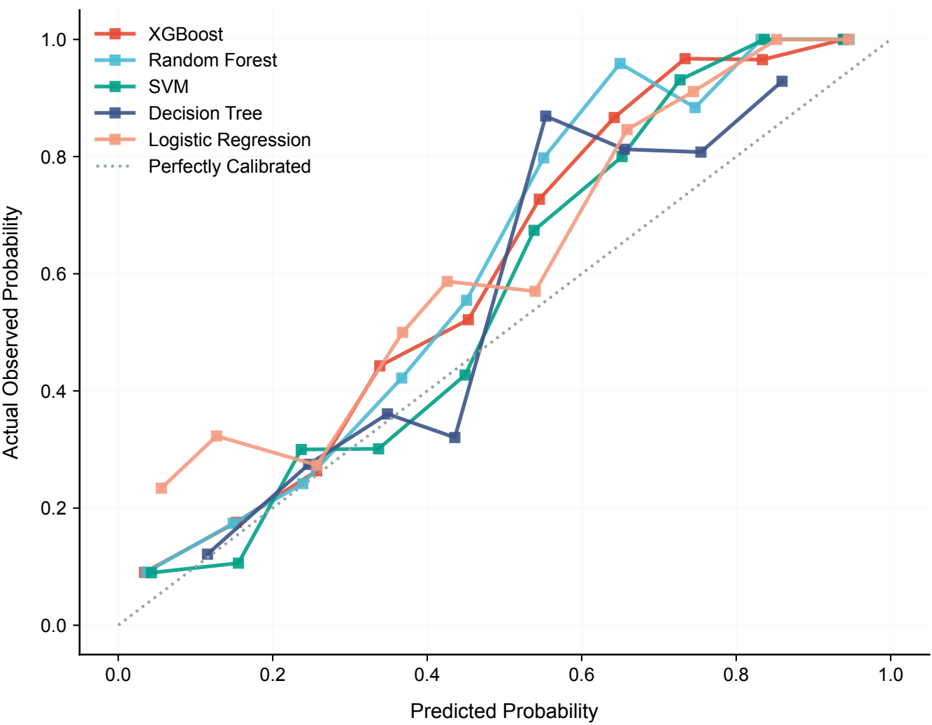
External Validation Calibration: POF (eICU)
