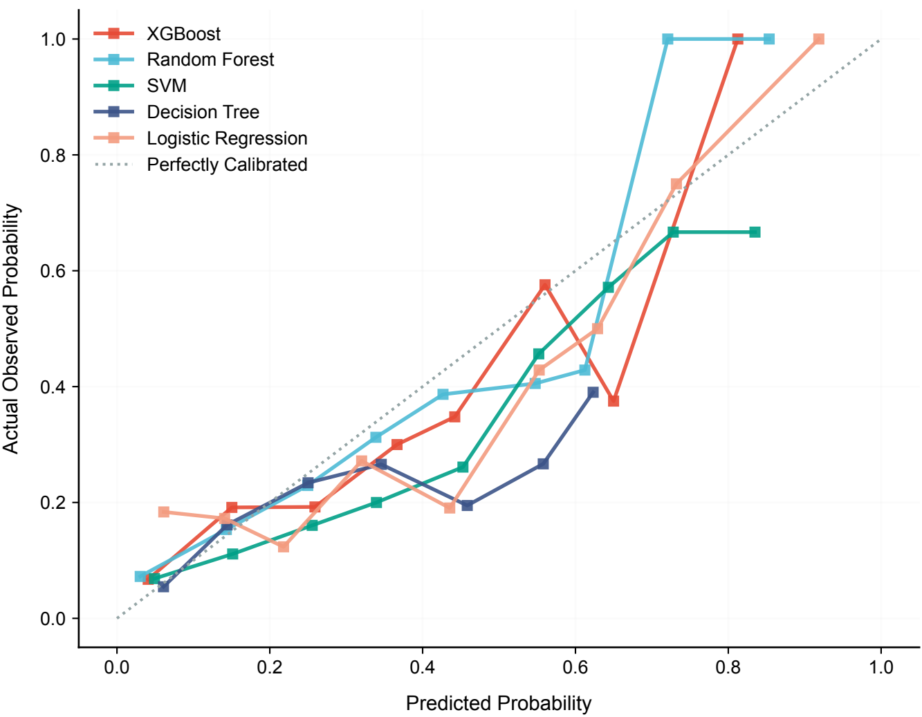
External Calibration: COMPOSITE (subgroup_no_renal = 1)
