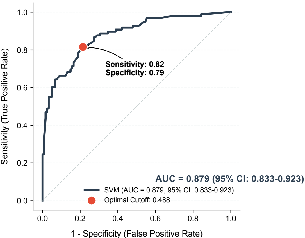
Diagnostic Performance: SVM (COMPOSITE)
