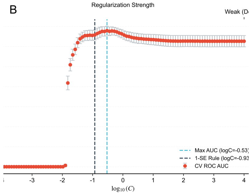
Predictors for MORTALITY
