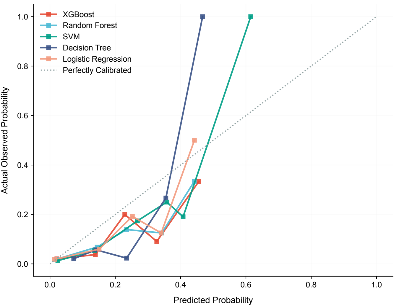
External Calibration: MORTALITY (subgroup_no_renal = 1)
