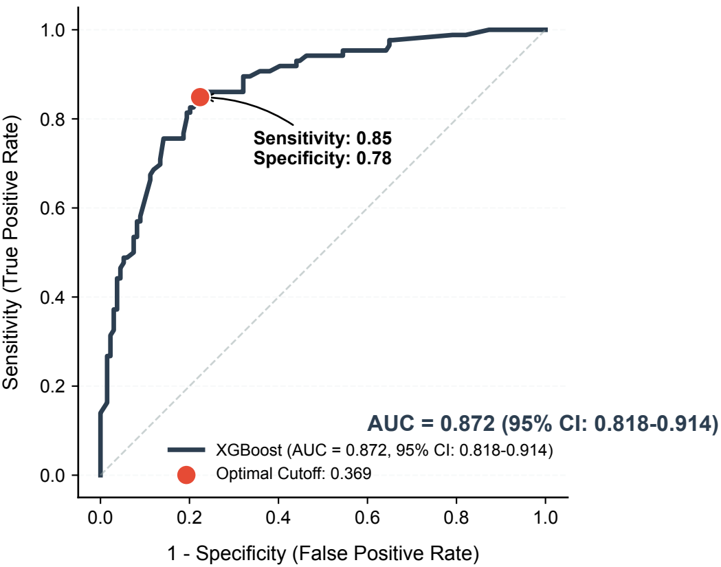
Diagnostic Performance: XGBoost (POF)
