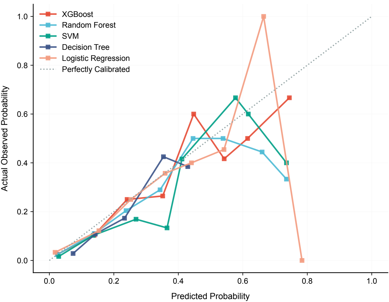
External Validation Calibration: MORTALITY (eICU)
