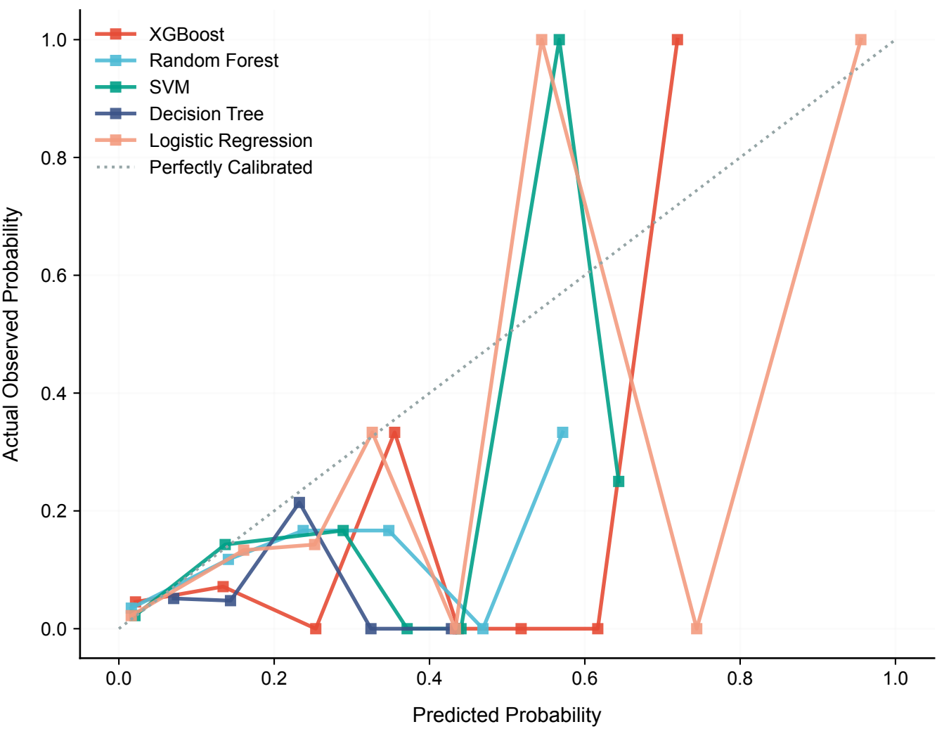
Calibration: MORTALITY (Subgroup No Renal = 1)
