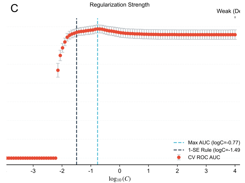
Predictors for COMPOSITE
