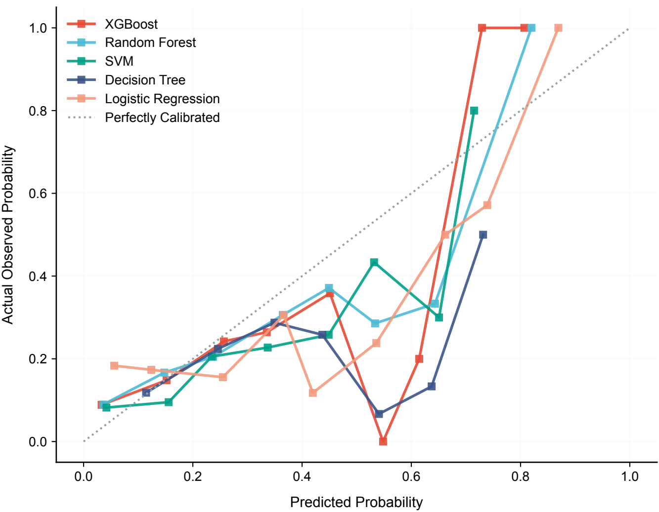
External Calibration: POF (subgroup_no_renal = 1)
