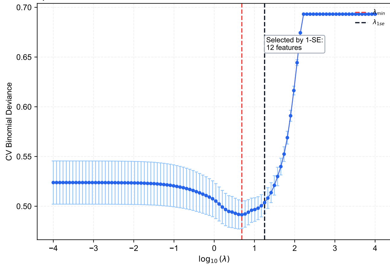
a) LASSO Cross-Validation Error Plot
