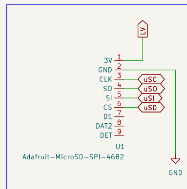
microSD SPI
