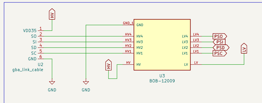
GBA Link Cable + Level Shifter
