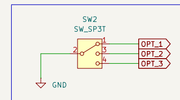
Payload Switcher
