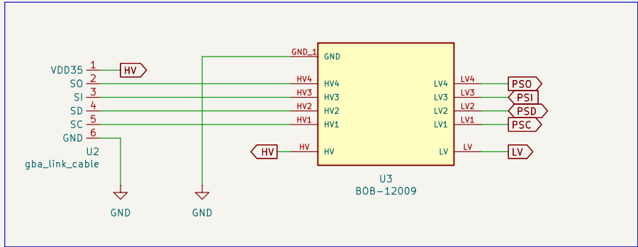
GBA Link Cable + Level Shifter
