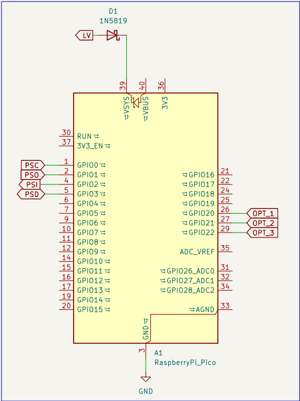
Raspberry Pi Pico
