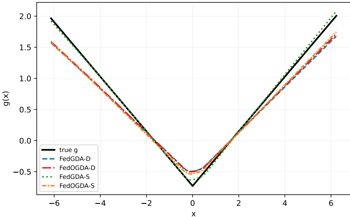
Absolute alpha=1.0 seed=0: all federated methods
