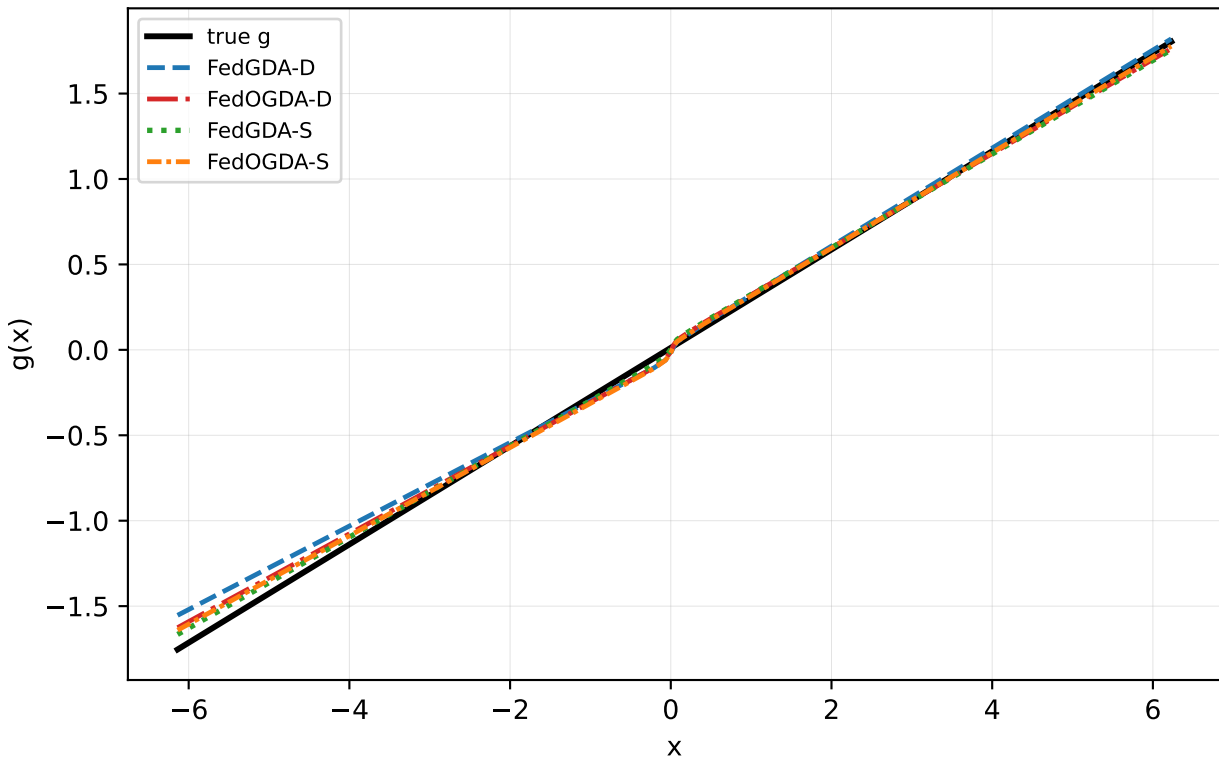
Linear \alpha=0.5 seed=1: all federated methods
