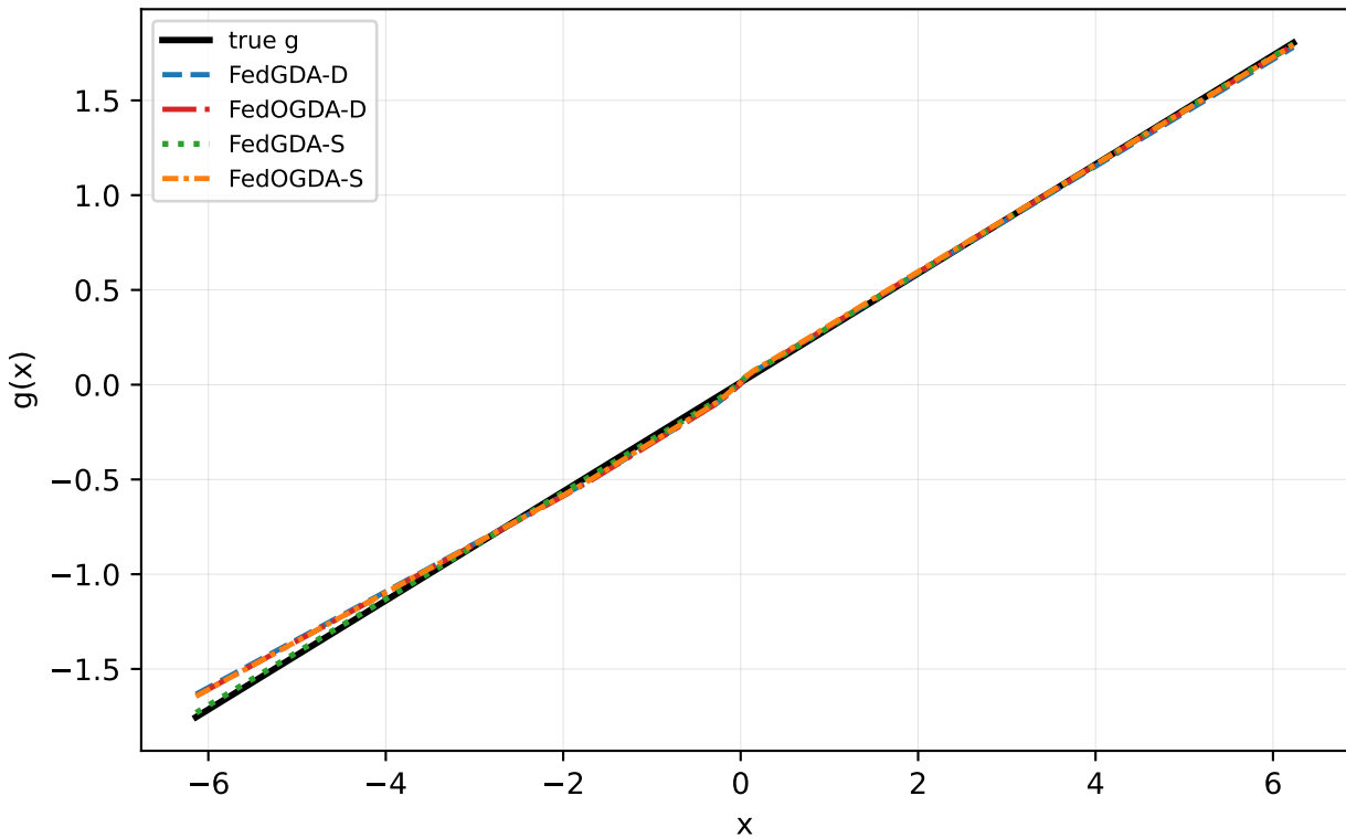
Linear alpha=1.0 seed=0: all federated methods
