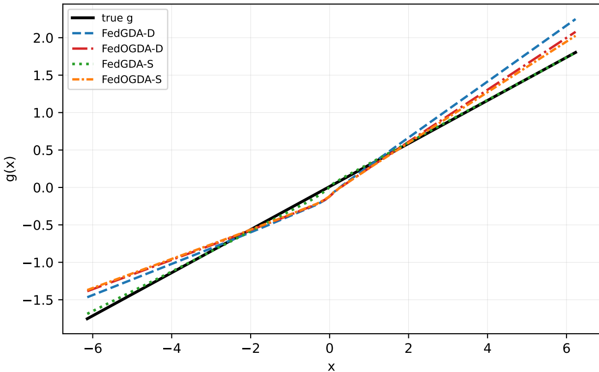
Linear alpha=1.0 seed=2: all federated methods
