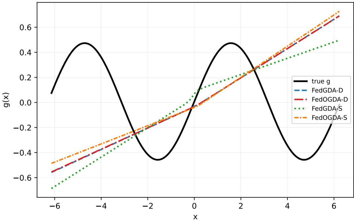
Sine \alpha=0.1 seed=0: all federated methods
