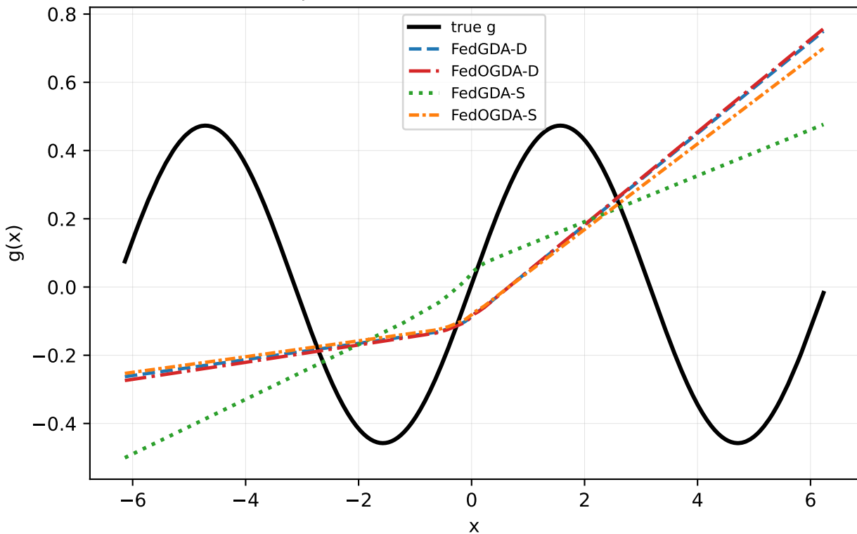
Sine \alpha=0.1 seed=2: all federated methods
