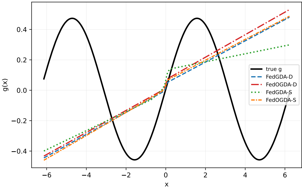
Sine \alpha=0.5 seed=1: all federated methods
