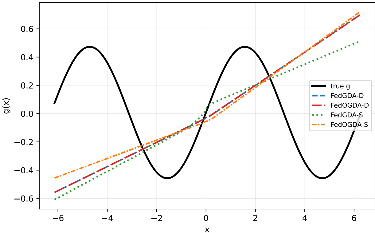
Sine \alpha=1.0 seed=0: all federated methods
