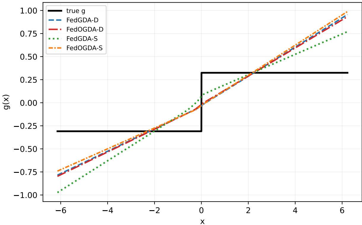
Step alpha=0.1 seed=0: all federated methods
