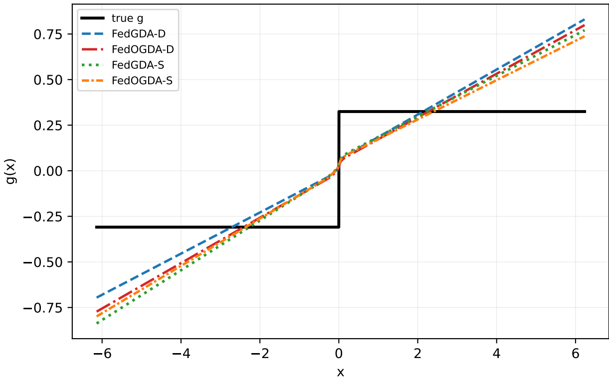
Step alpha=0.1 seed=1: all federated methods
